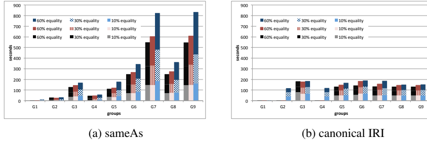
Fig. 3: Execution times of most expensive queries with 2 datasets
