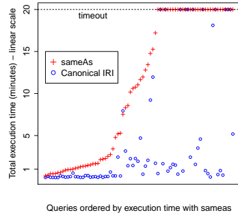
Fig. 2: Execution time and statistics for the queries in the federated setting at Statoil
