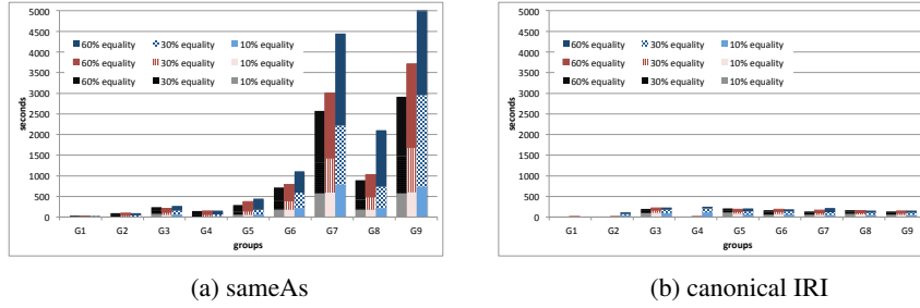
Fig. 4: Execution times of most expensive queries with 3 datasets
